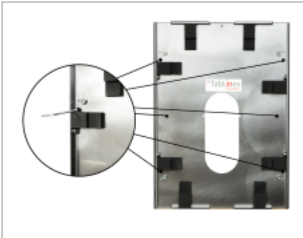
Fig. 4: The Tablet holder remains adjustable after tightening; Correcting bumps using M5 screws
