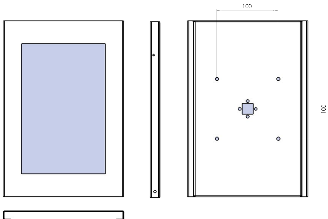
Fig. 1: VESA mounting of TabLines TSG tablet protective housing
