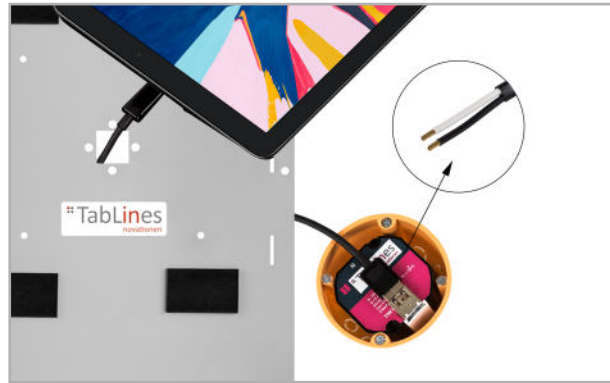
Fig. 7: Connect tablet with optional power supply unit
