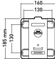
Wall mount
