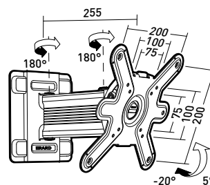
Mounting plate
