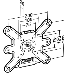
Mounting plate
