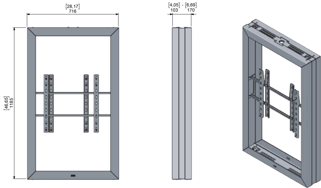
Technical drawing (mm/inch) Casing Complete Top Mounted Back to Back 48-49"
