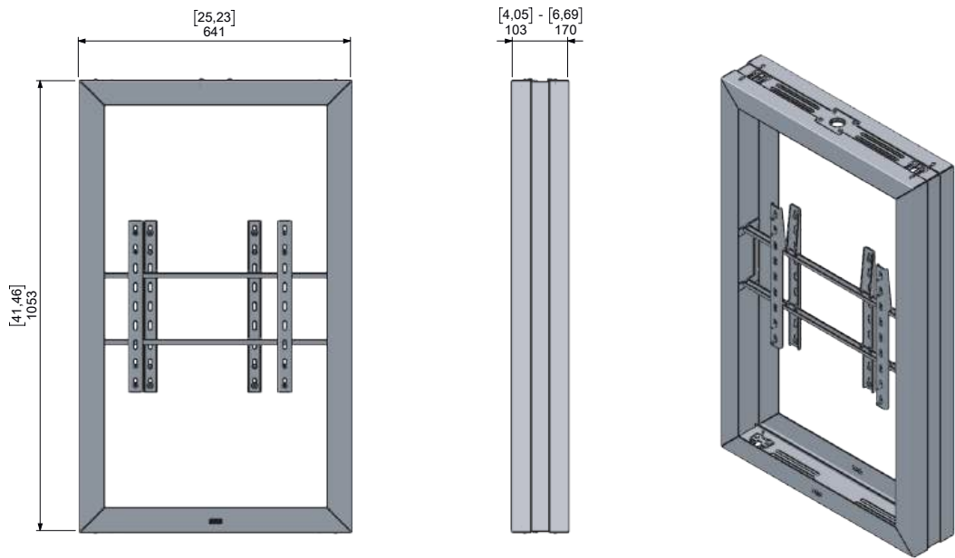
Technical drawing (mm/inch) Casing Complete Top Mounted Back to Back 42-43"
